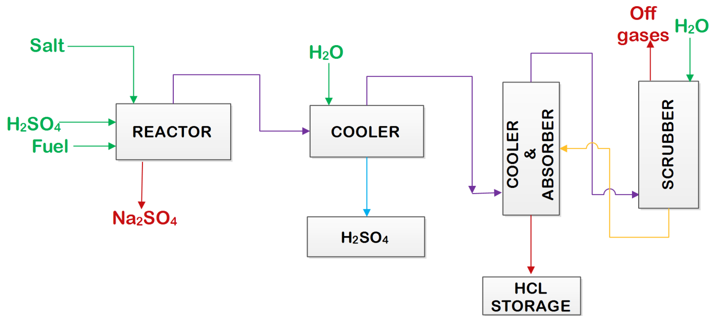
Figure: Manufacturing of Hydrochloric acid from salt & sulfuric acid
